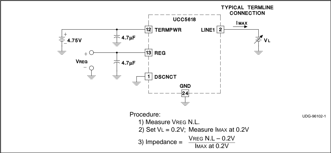
Figure 1. Termline Impedance Measurement Circuit
